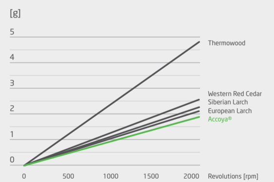
TABER ABRASION WEIGHT LOSS
